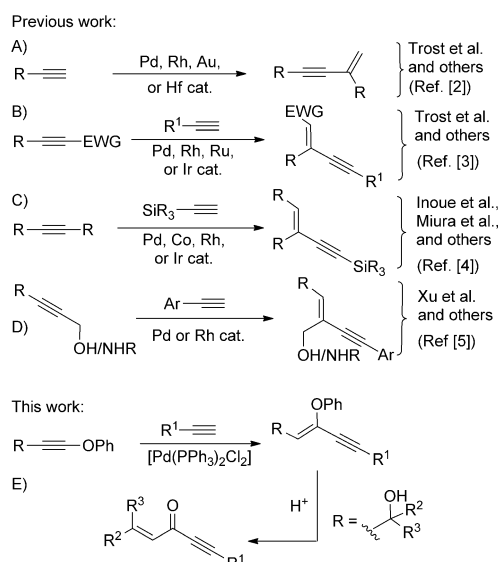
Scheme 1. Alkyne–alkyne cross-addition.
